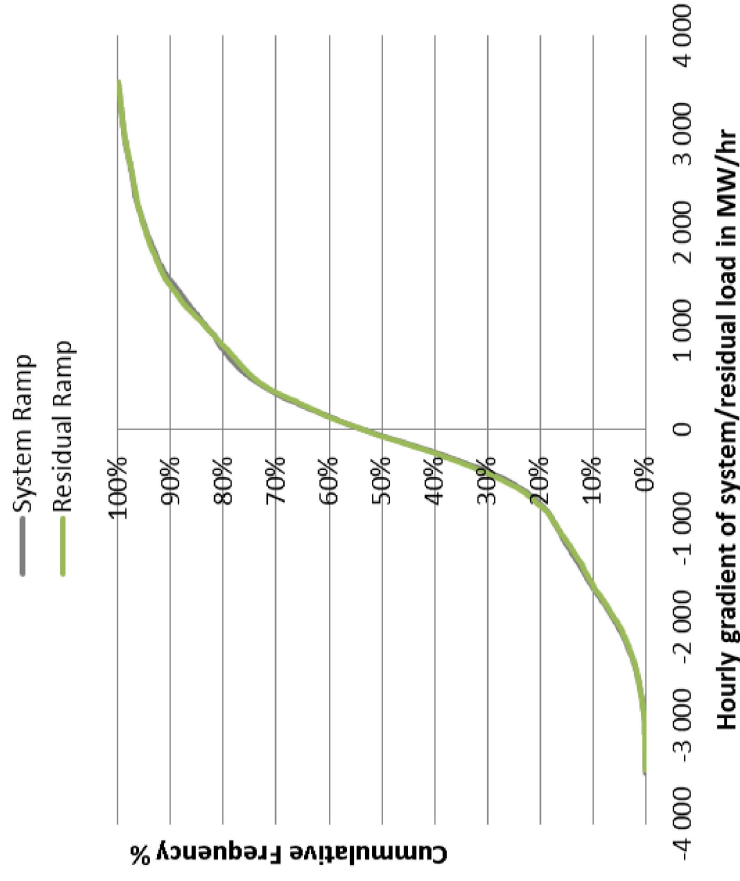
Cumulative frequency distribution of 1-hour gradients for all hours from Jan – Dec 2016
