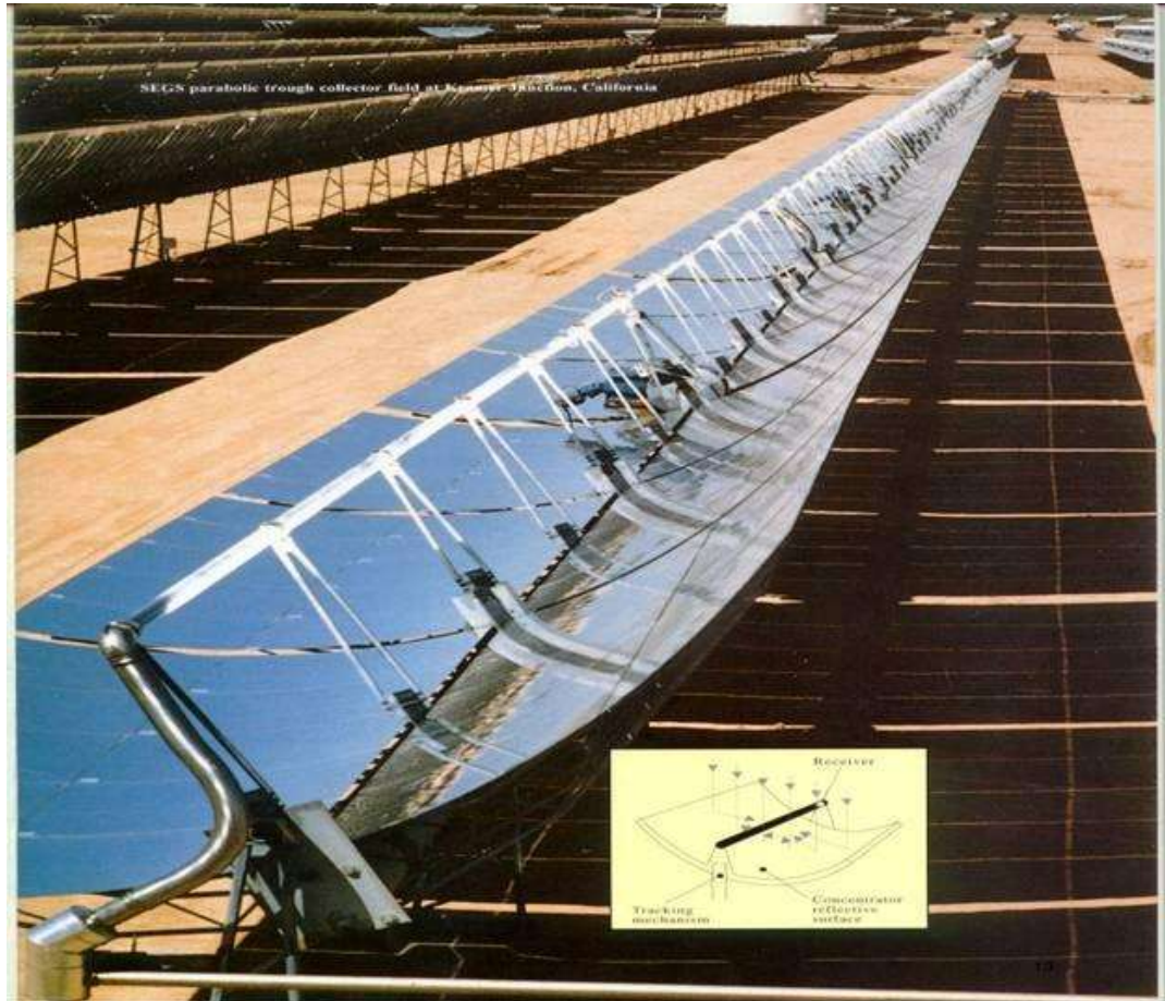
Figure 5-3: Trough collectors
