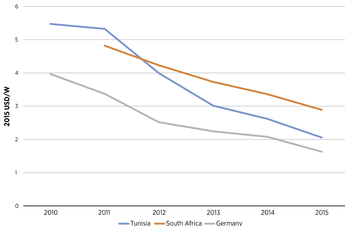
FIGURE 25: COMPARISON OF AVERAGE TOTAL INSTALLED COST OF RESIDENTIAL SOLAR PV SYSTEMS, 2010-2015
