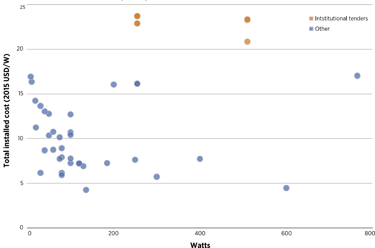
FIGURE 15: SMALL SOLAR HOME SYSTEM (&lt;1 kW) COSTS BY SYSTEM SIZE IN AFRICA, 2012-2015
