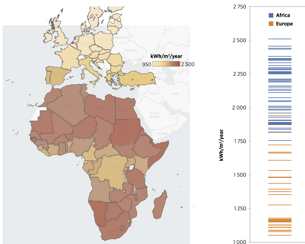
FIGURE 10: SOLAR RESOURCE ON AN OPTIMALLY SLOPED SURFACE IN EUROPE AND AFRICA
