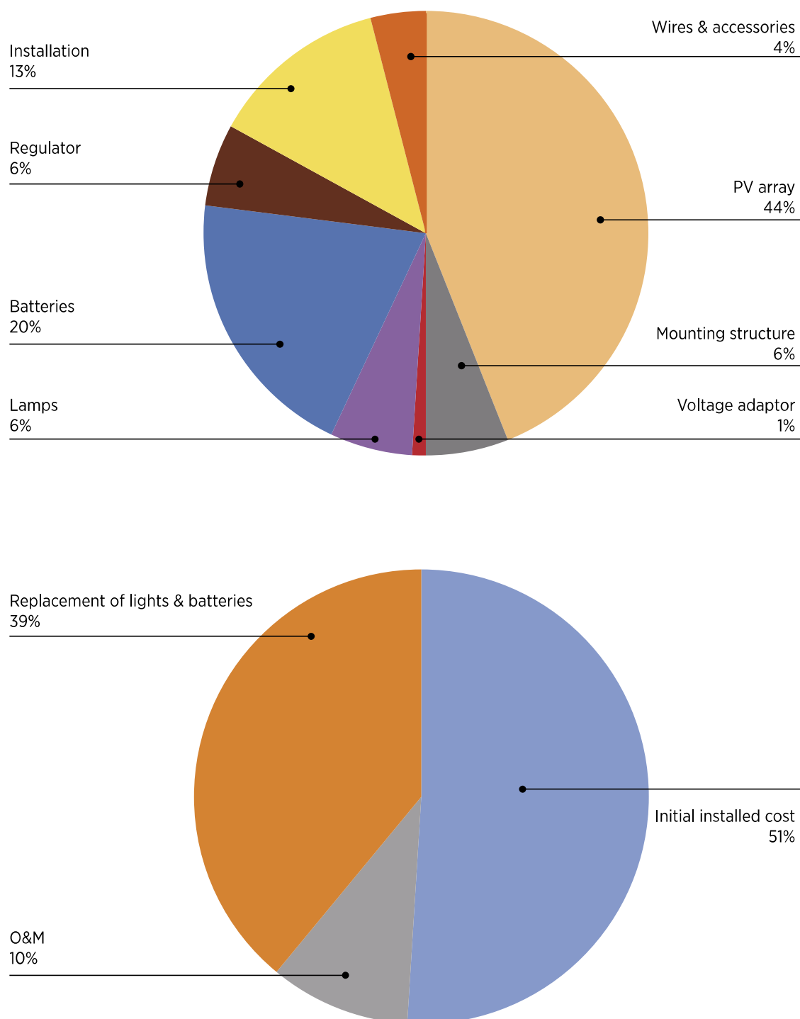
FIGURE 26: COST BREAKDOWN OF 100 Wp SOLAR PV SYSTEM (ABOVE) AND ANNUALISED LIFE-CYCLE COST (BELOW) IN GHANA
