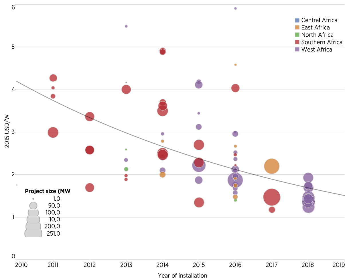
FIGURE ES 1: OPERATING AND PROPOSED UTILITY-SCALE SOLAR PV PROJECT INSTALLED COSTS IN AFRICA, 2011-2018
