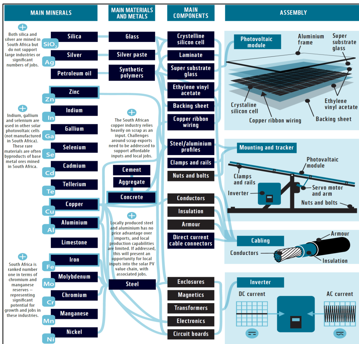
Figure 4: Materials and manufacturing value chain for solar PV – Opportunities for South Africa
