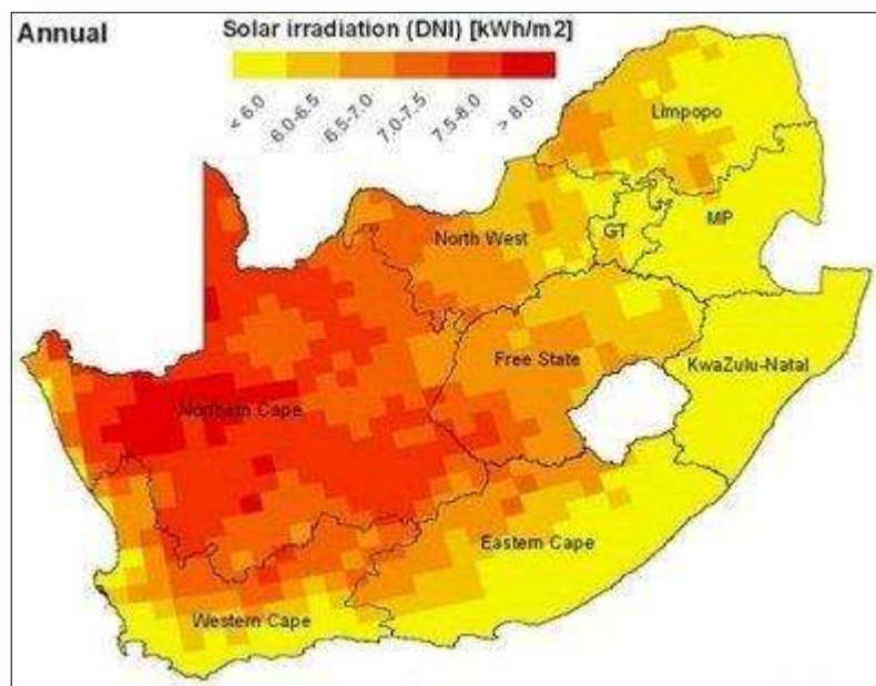
Figure 1-4: Solar radiation in SA
