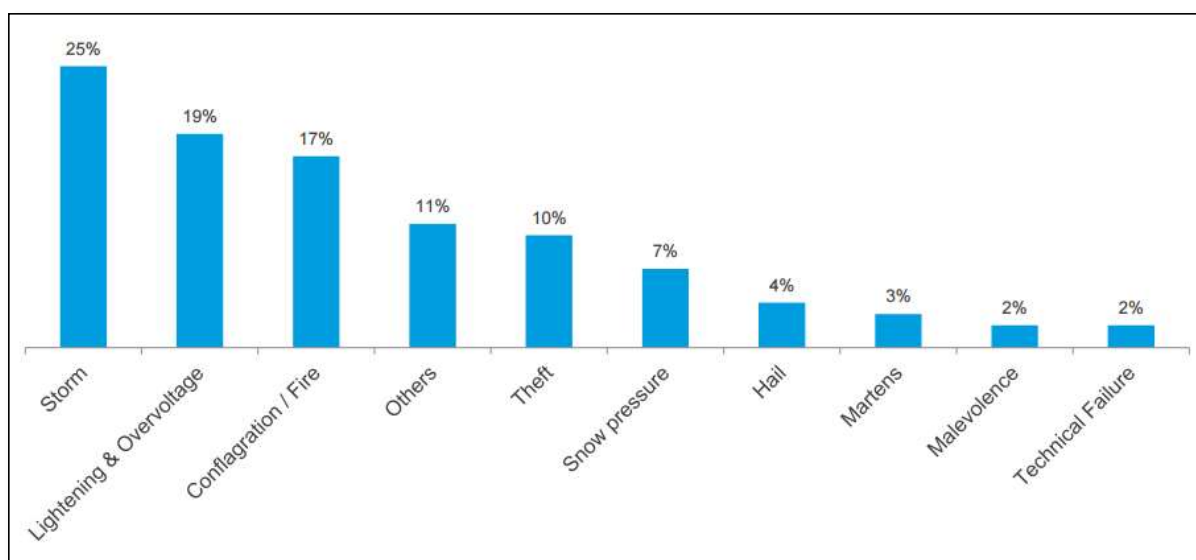
Figure 2-17: Causes of insurance claims – Germany 2003 to 2008
