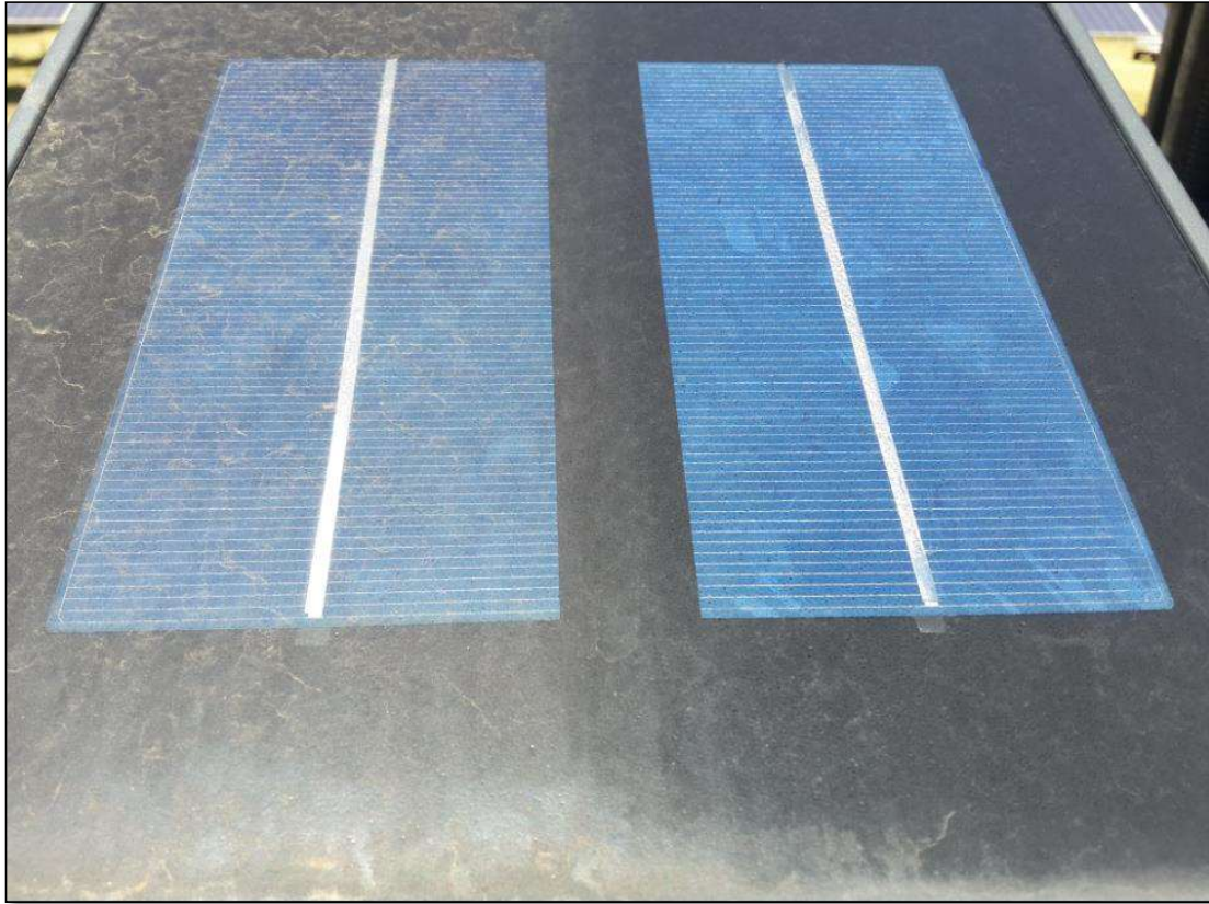
Figure 2-7: Reference cells
