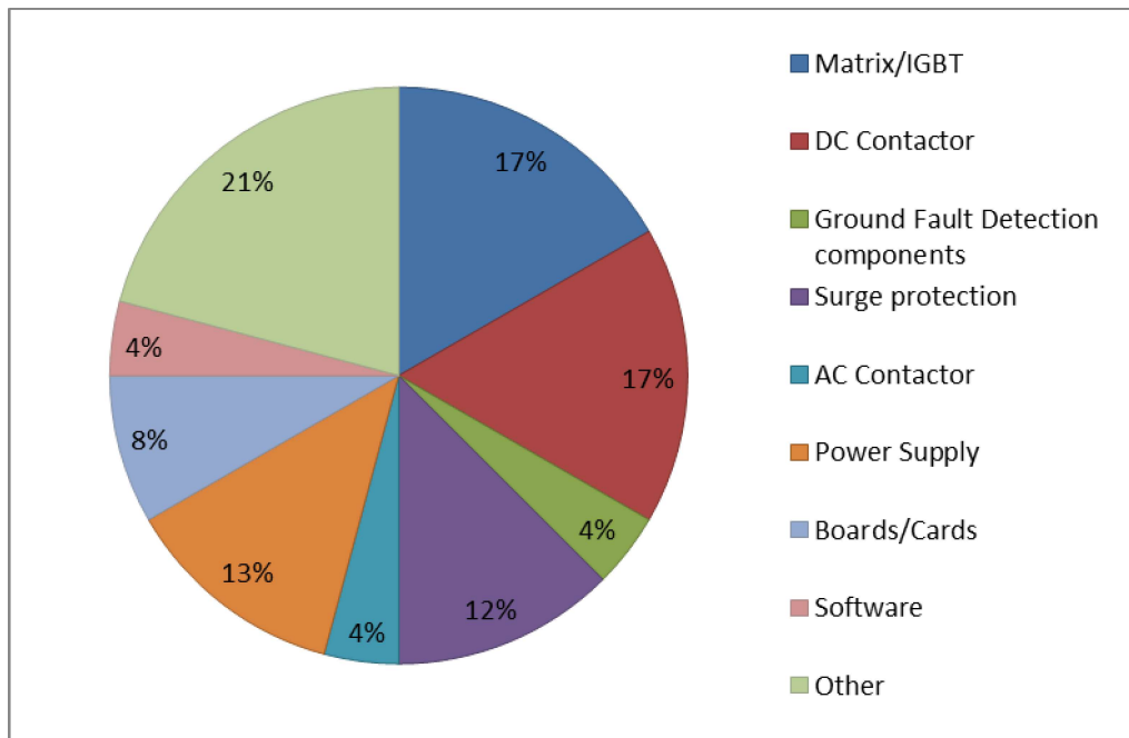
Figure 3-6: Inverter faults
