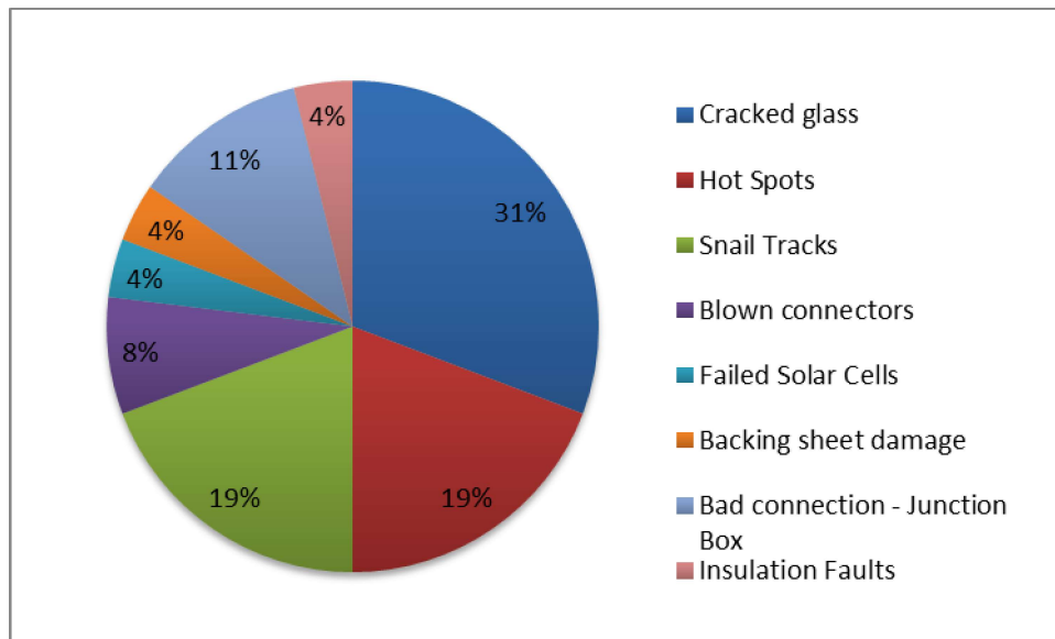
Figure 3-3: PV module defects
