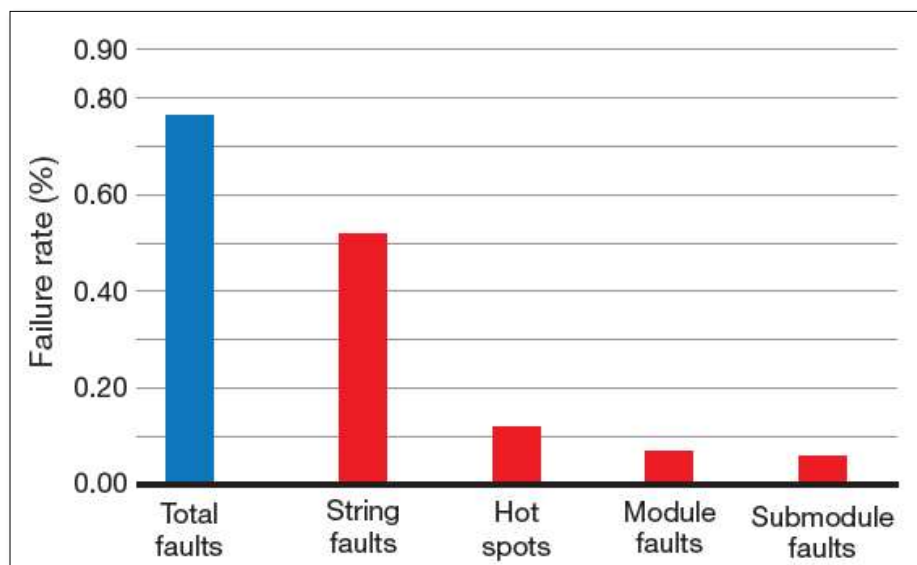
Figure 2-14: Failures in PV strings
