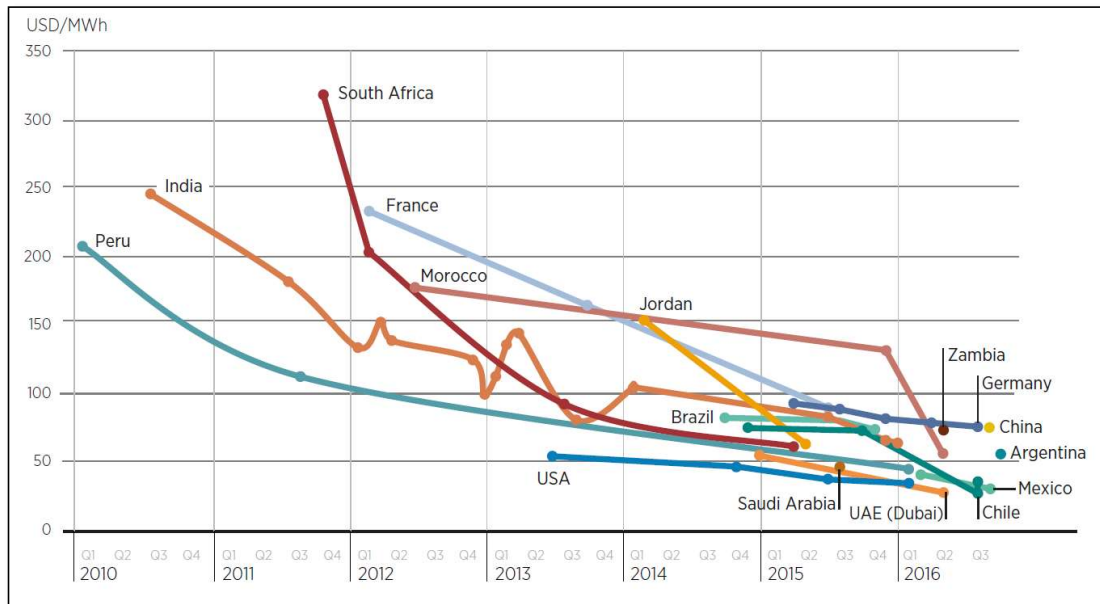
Figure 2-8: Utility scale solar PV bid prices from around the world
