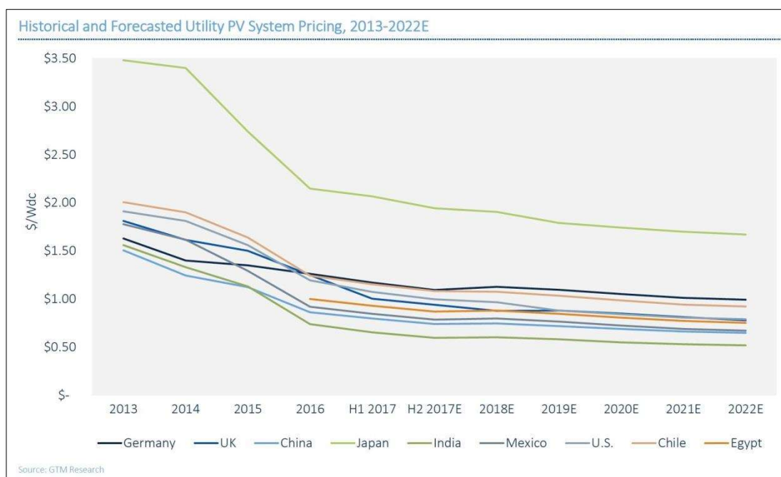
Figure 3-16: Historical and forecasted utility PV system pricing Source: Wesoff and Lacey (2017)
