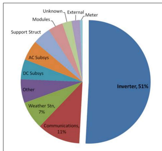
Figure 2-15: Failures in SunEdison operated and maintained PV plants (2008 to 2010)
