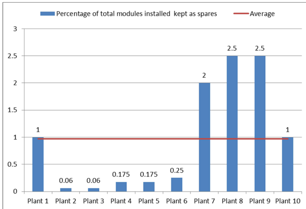
Figure 3-4: Percentage of total modules installed kept as spares
