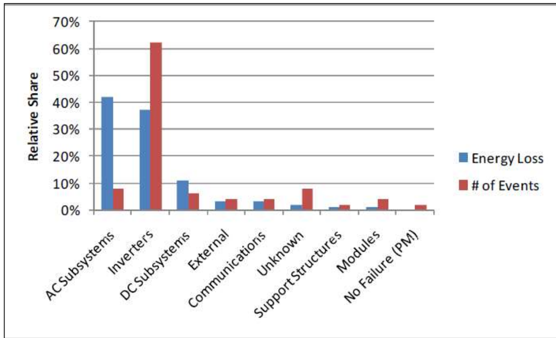
Figure 2-1: Relative frequency of failure of PV components
