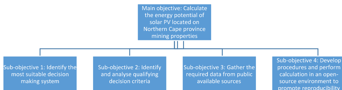
Figure 1. Research objectives.
